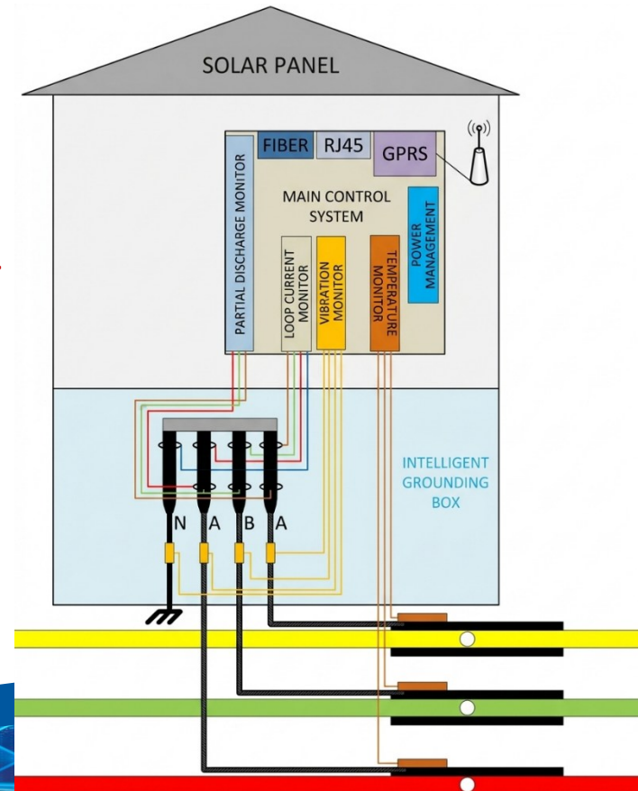
Intelligent Grounding Unit (IGUHV) for High Voltage Cables
